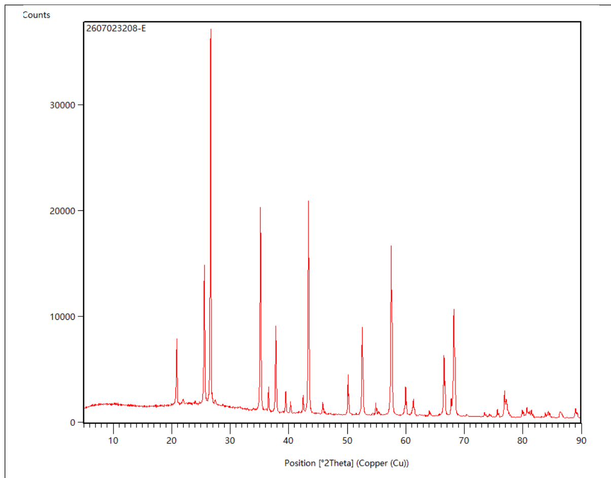
Fig.2: XRD spectrum
