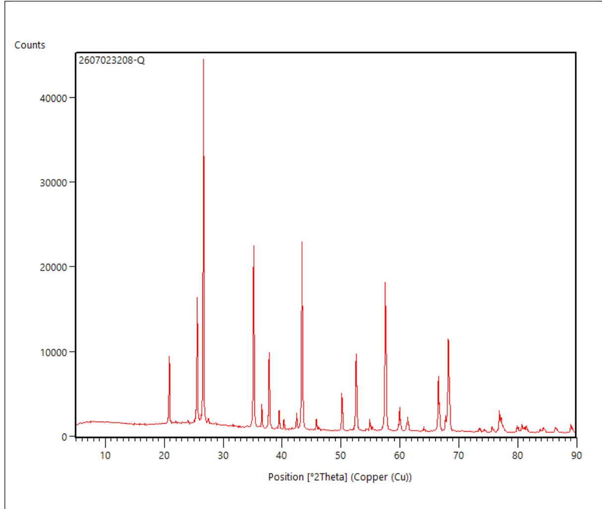
Fig.2: XRD spectrum
