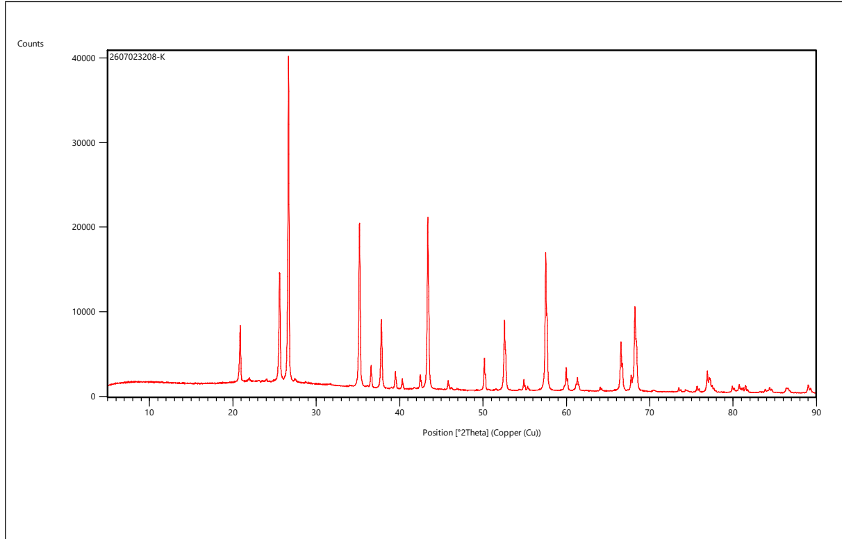
Fig.2: XRD spectrum
