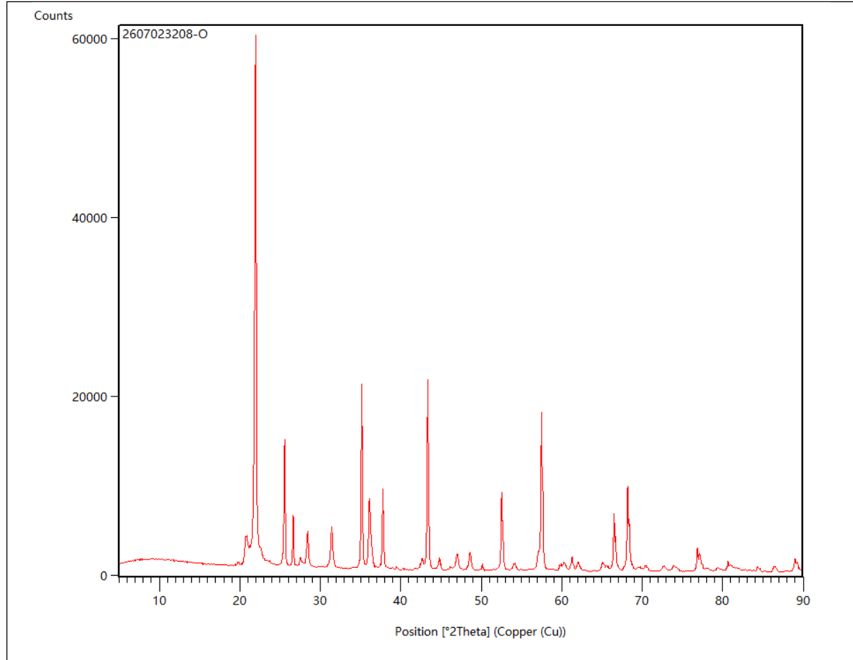
Fig.2: XRD spectrum
