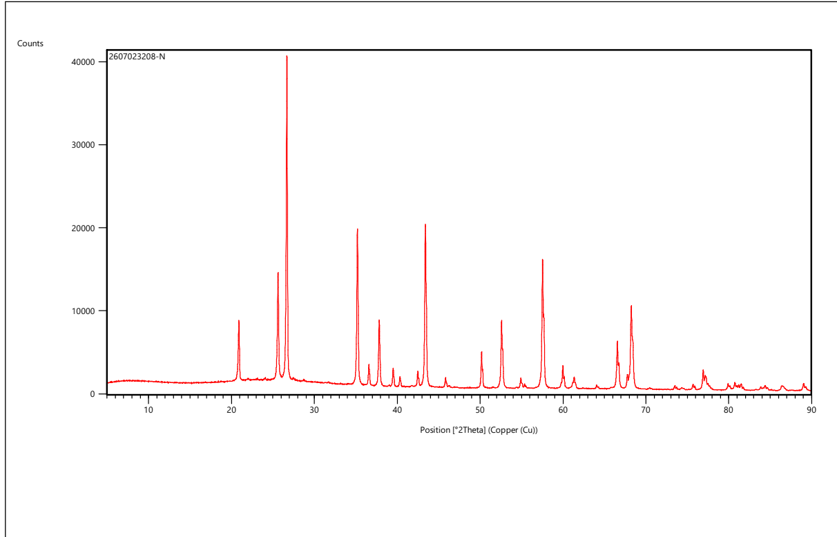
Fig.2: XRD spectrum
