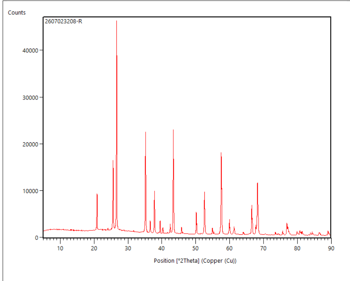
Fig.2: XRD spectrum
