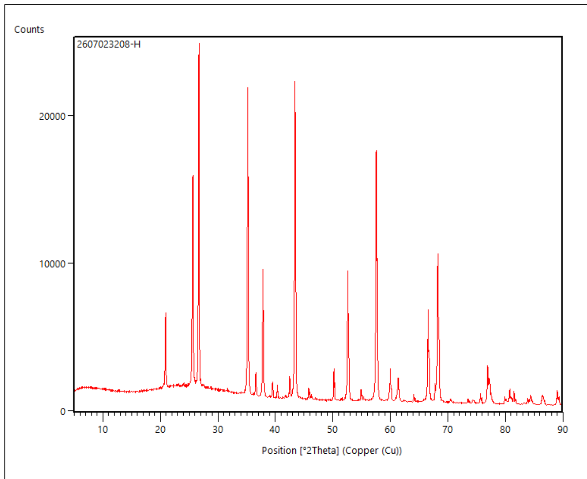
Fig.2: XRD spectrum
