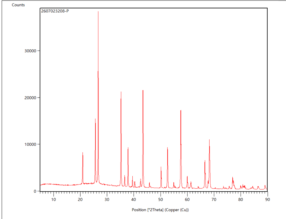
Fig.2: XRD spectrum
